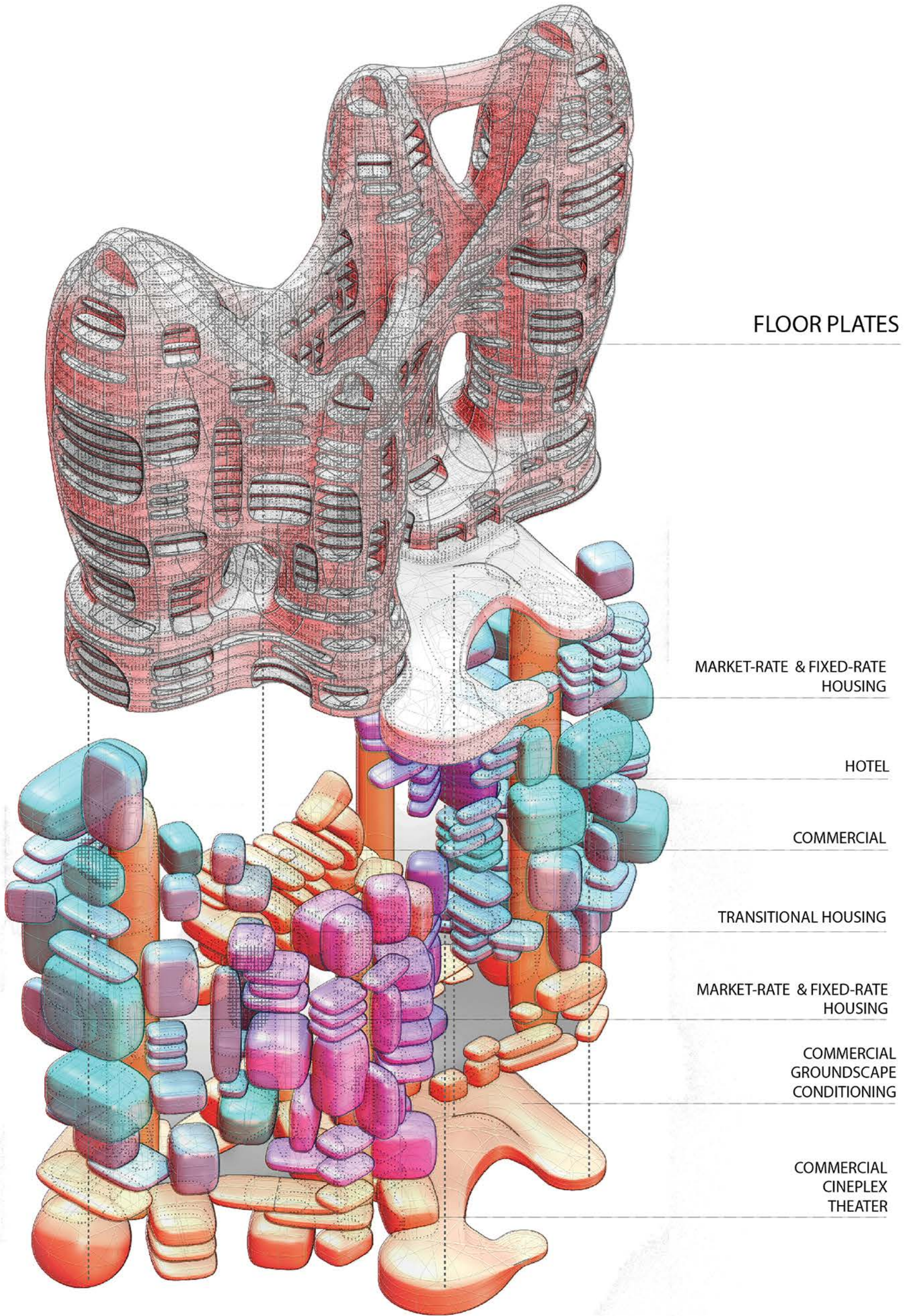
EXPLODED AXON DIAGRAM
